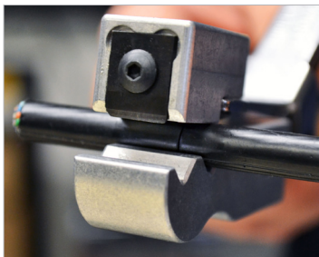
Factory-set, non-adjustable ringing blade accurately slices through the jacket depth without fiber damage.
